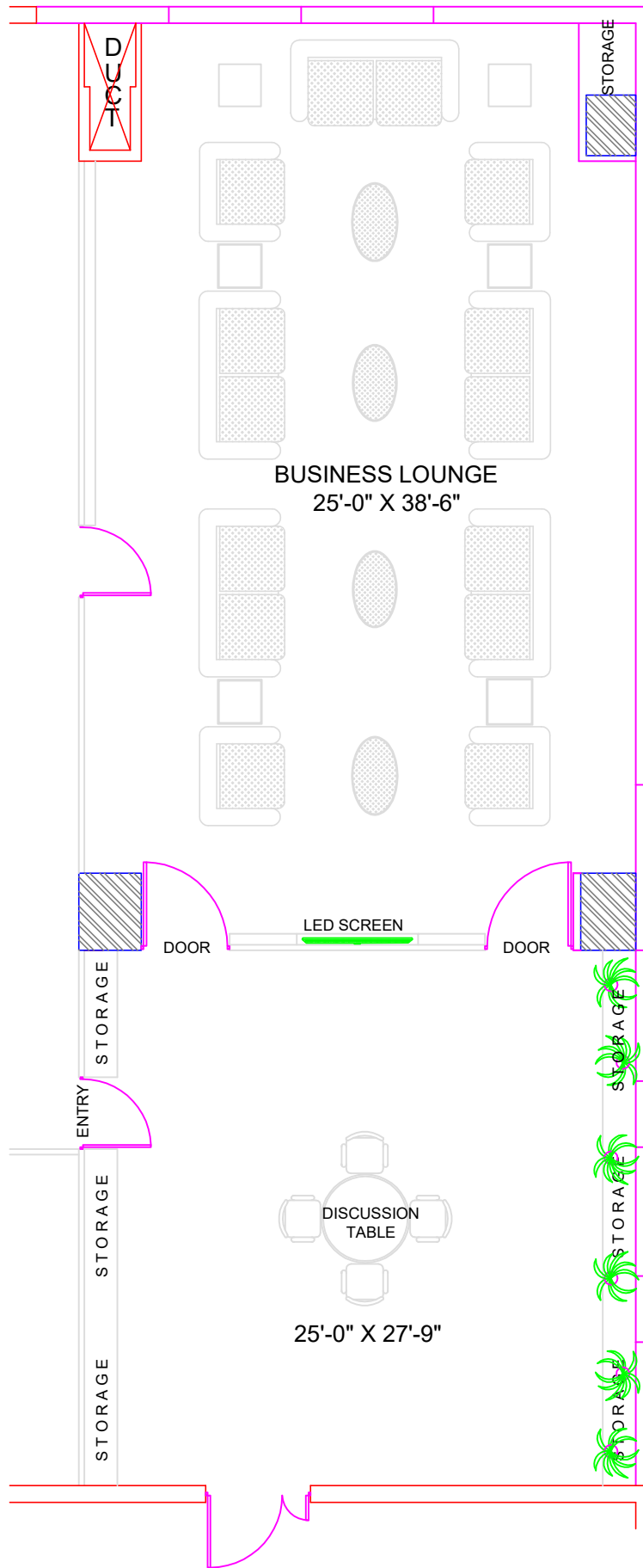
10TH FLOOR PLAN (PART) ALTERNATIVE - 10
